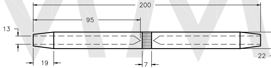
ALUMINIUM COMPRESSION SLEEVE
